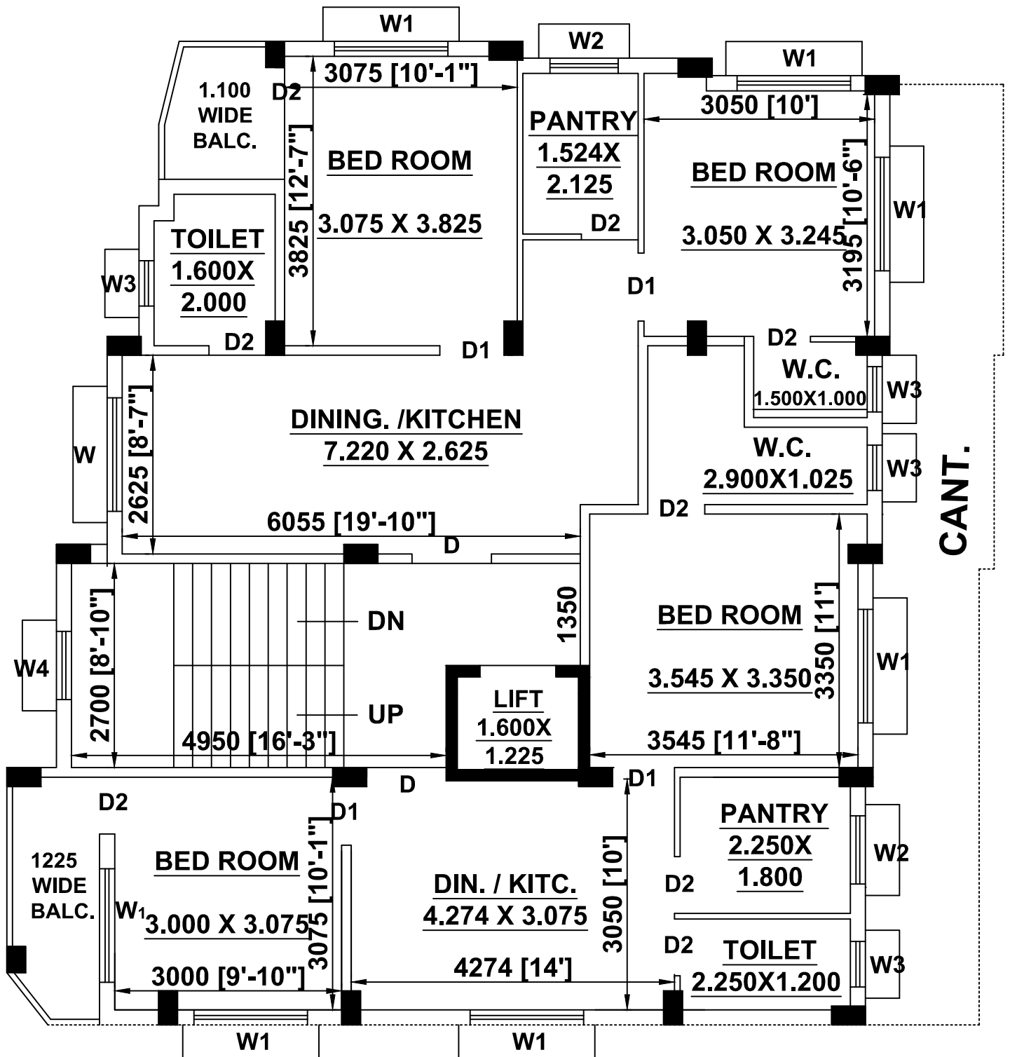
PROP. FIRST FLOOR PLAN (1:1)
